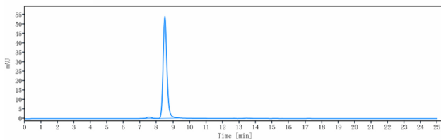
SEC-HPLC
