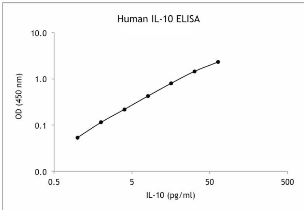
Example of a representative Human IL-10 standard curve using a 4-parameter logistic fit.
