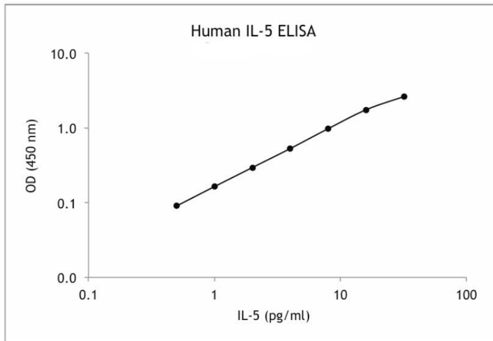
Example of a representative Human IL-5 standard curve using a 4-parameter logistic fit.
